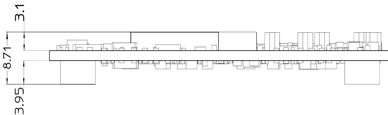
Fig. 5: Board layout - size view
